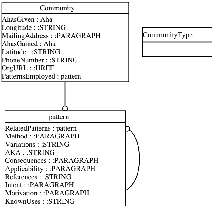
UML Class Diagram for communities_ontology
