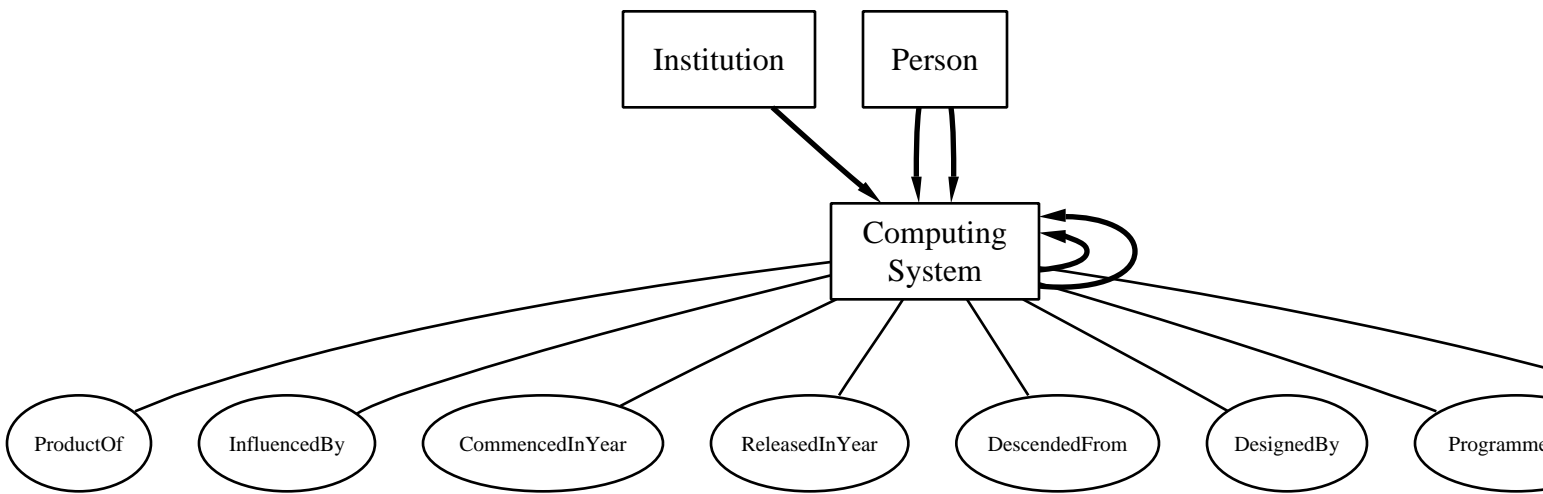
Entity Relationship Diagram for computing_systems_data
