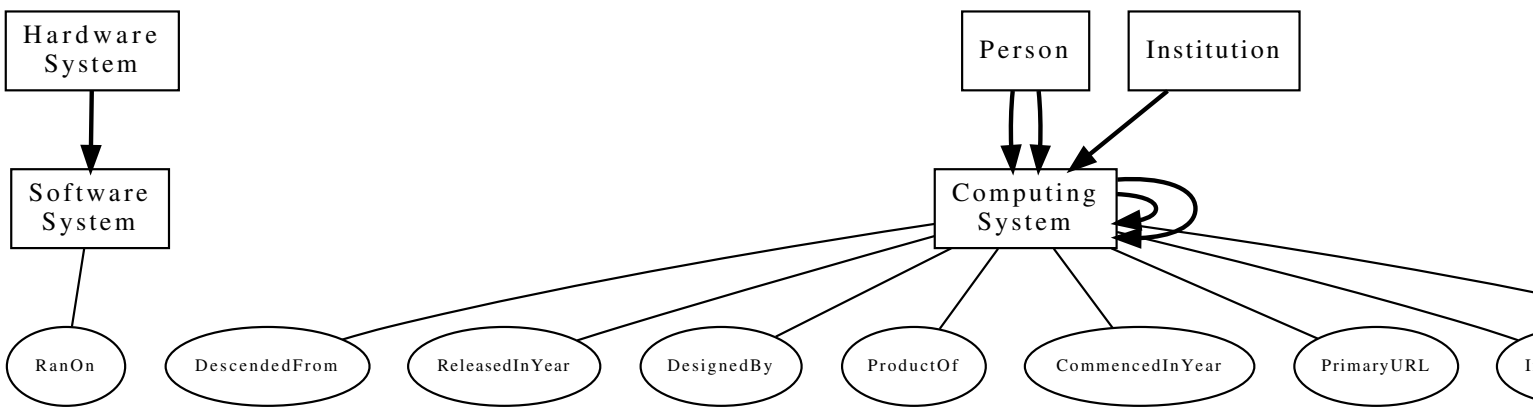
Entity Relationship Diagram for Computing Systems Ontology
