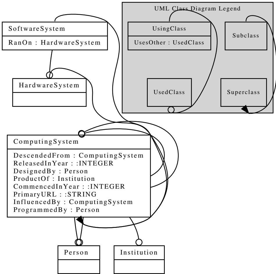
UML Class Diagram for Computing Systems Ontology
