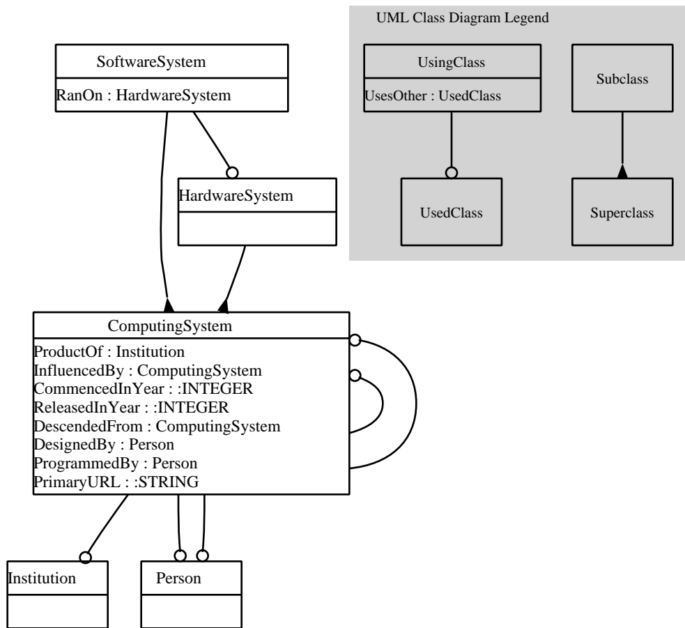
UML Class Diagram for Computing Systems Ontology
