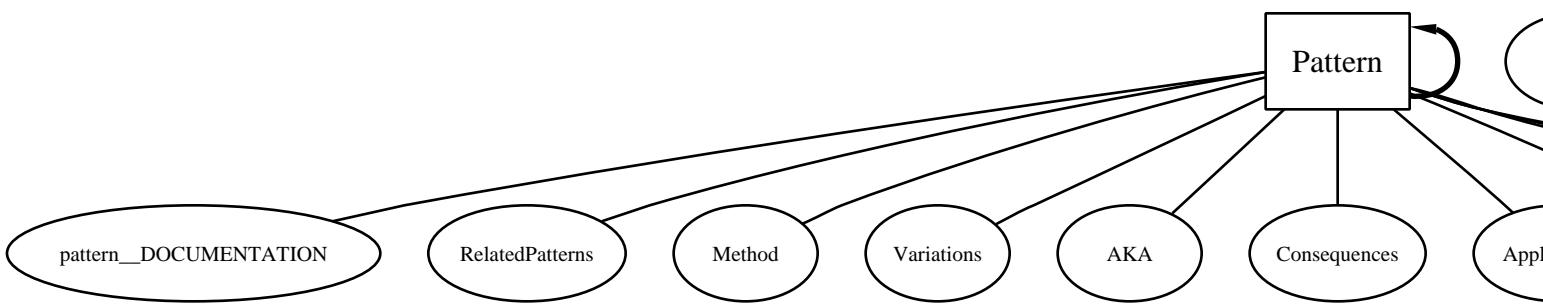
Entity Relationship Diagram for The Conversation Pattern
