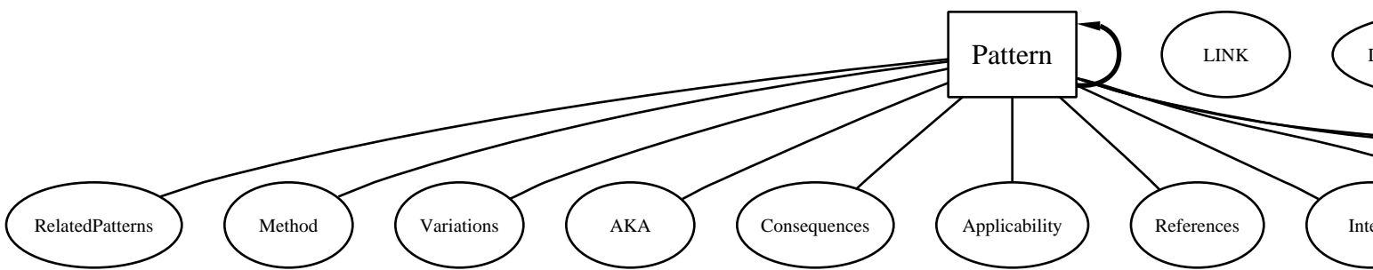
Entity Relationship Diagram for conversation_pattern_la
