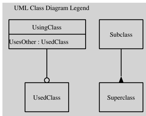
UML Class Diagram for faq_ontology
