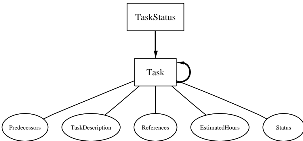
Entity Relationship Diagram for nooron_pert_data
