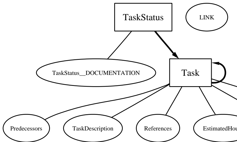
Entity Relationship Diagram for nooron_project_data
