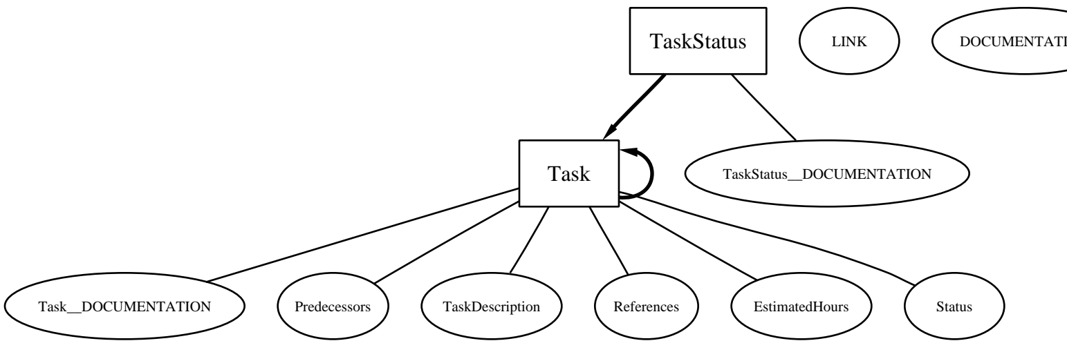
Entity Relationship Diagram for pert_wardrobe
