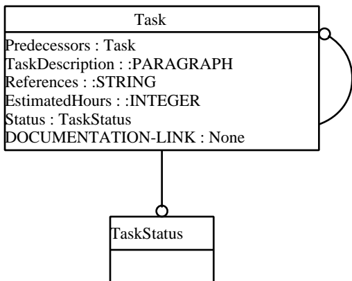
UML Class Diagram for Project Management
