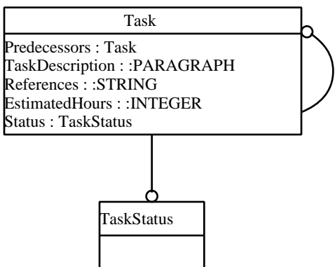
UML Class Diagram for Project Management
