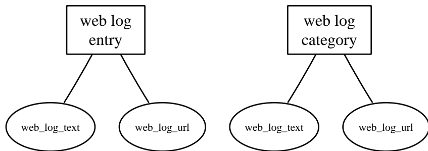
Entity Relationship Diagram for smurp's blog
