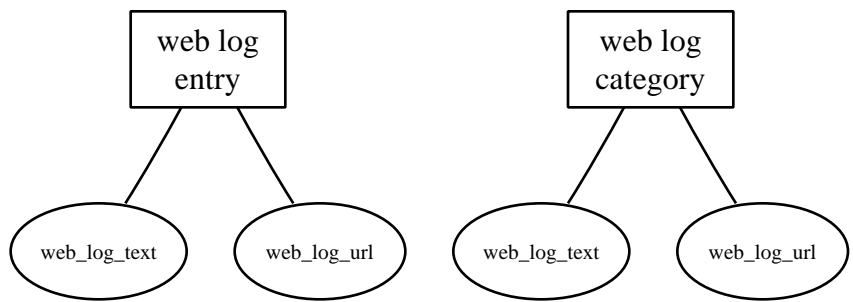
Entity Relationship Diagram for smurp_web_log_data
