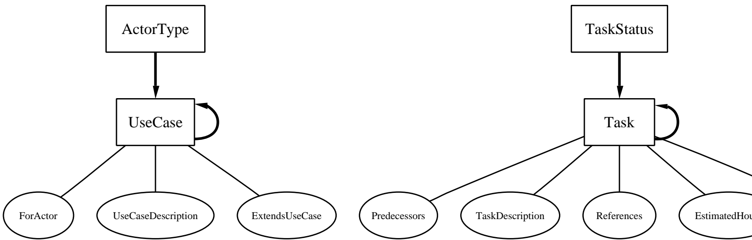
Entity Relationship Diagram for Software Project Management
