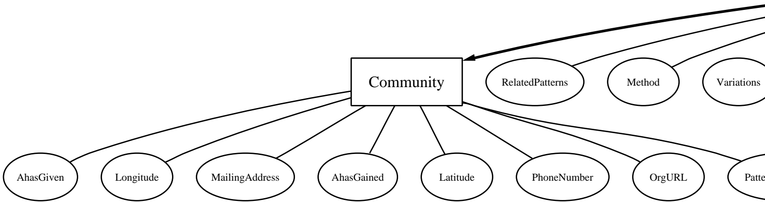
Entity Relationship Diagram
