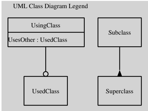
UML Class Diagram for web_log_ontology
