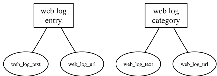
Entity Relationship Diagram for web_log_wardrobe
